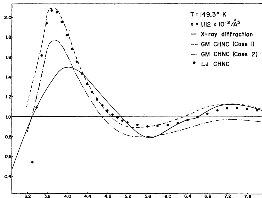
FIG. 16. The computed g 's from the CHNC equation with the GM and LJ potentials at 149.3°K. Case 1 and case 2 correspond to two different solutions obtained with the GM potential. The x-ray diffraction curve is due to Eisenstein and Gingrich.
