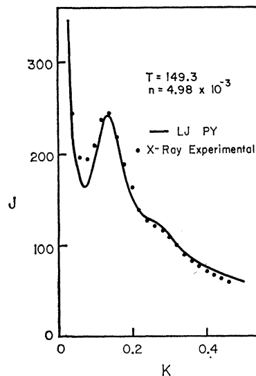
FIG. 29. The computed J 's from the PY equation with the GM and LJ potentials at 149.3°K. The x-ray diffraction points are due to Eisenstein and Gingrich. The J^2 ( f is atomic structure factor) curve is also plotted.
