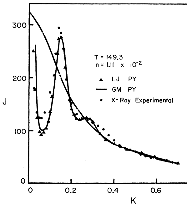
FIG. 29. The computed J 's from the PY equation with the GM and LJ potentials at 149.3°K. The x-ray diffraction points are due to Eisenstein and Gingrich. The J^2 ( f is atomic structure factor) curve is also plotted.
