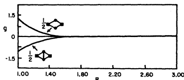
FIG. 3. The contributions due to the elementary and composite diagrams with two field points. (From Klein's thesis.)
