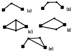
FIG. 2. One and two field points diagrams included in s(r) or [s(r)]^2 .
