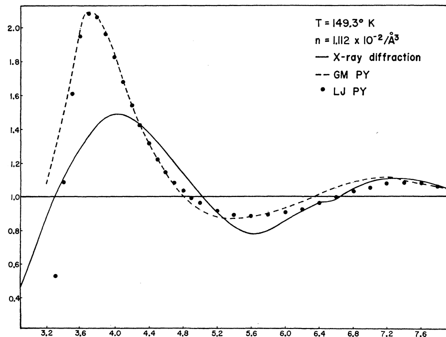
FIG. 17. The computed g 's from the PY equation with the GM and LJ potentials at 149.3°K. The x-ray diffraction curve is due to Eisenstein and Gingrich.
