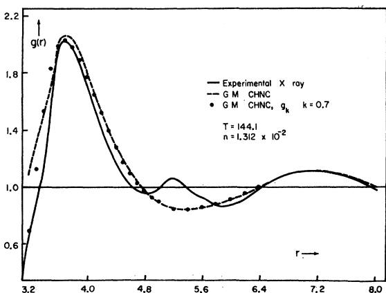
FIG. 33. The dashed curve is the g computed from the CHNC equation with the GM potential. The g_k is shown by the dots. (Maximum value of K used for the computation of g_k is 0.7.) The x-ray diffraction curve is due to Eisenstein and Gingrich.
