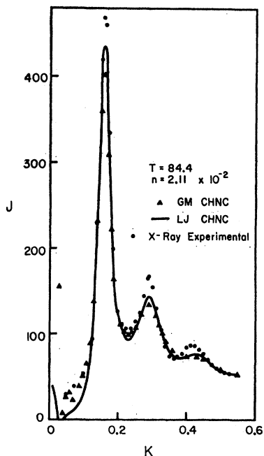
FIG. 19. The computed J 's from the CHNC equation with the GM and LJ potentials at 84.4°K. The x-ray diffraction points are due to Eisenstein and Gingrich.
