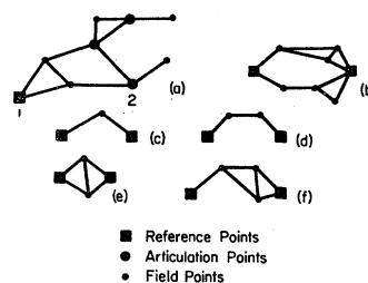
FIG. 1. Reducible diagram, (a); irreducible diagrams, (b, c, d, e, f); reference points, articulation points, and field points. Simple diagrams, (c, d, e, f); composite diagram, (b).
